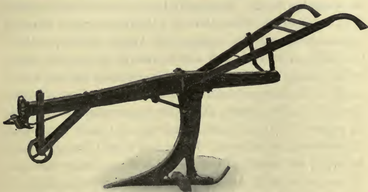
5. A SUBSOIL PLOW
